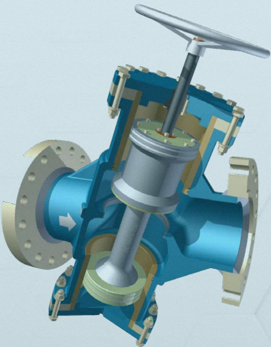
ILLUSTRATION OF THE HYDROCORE VALVE WITH ONLY ONE MOVEABLE PART
