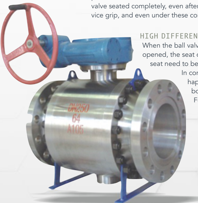
BALL VALVE ILLUSTRATION
